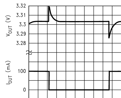
Load Transient Response ( C_{OUT} = 2.2\mu F )
